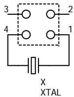
Dip Meter K-126C(Kyoritsu) Original Schematic Diagram
